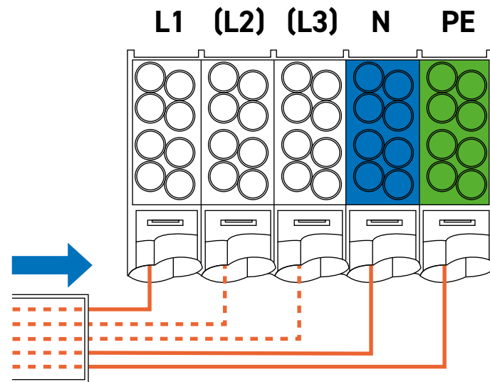
SUPPLY CABLE
