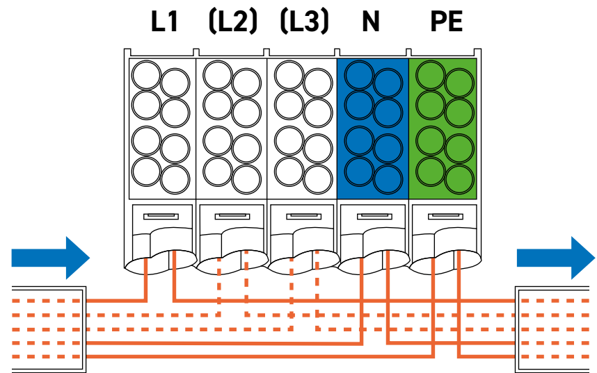
SUPPLY CABLE
