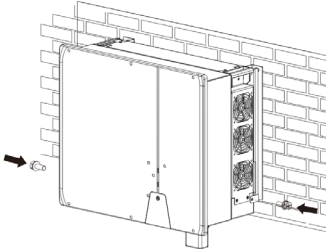
Fig. 8.1: Securing the inverter
