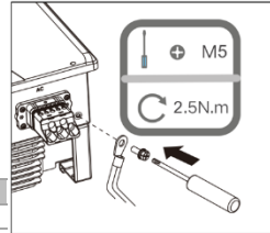
Fig. 17: Connecting grounding
