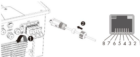
Fig. 20: Insert the network cable
