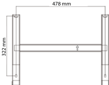
Fig. 4: Hull for vegghmontering
