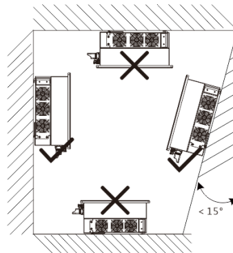
Fig. 2: Permissible installation location
