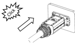
Fig. 12: Press the cover
