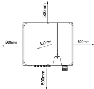
Fig. 3.1: Device for outdoor installation
