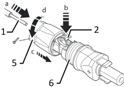
Fig. 14: Introducerea firelor
